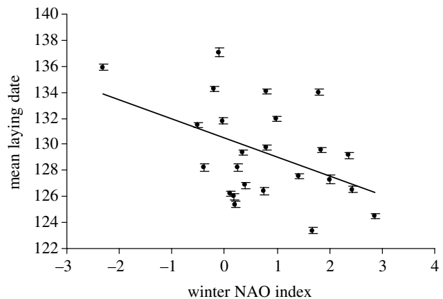
Figure 1. Annual mean laying date in the colony, in number of days since January 1 ( \pm s.e.), plotted against NAO values for each year, showing a significant negative relationship ( b=-1.56 \pm 0.59 , R^2=0.24 , p=0.015 ). This effect of NAO on laying date is independent of year.
